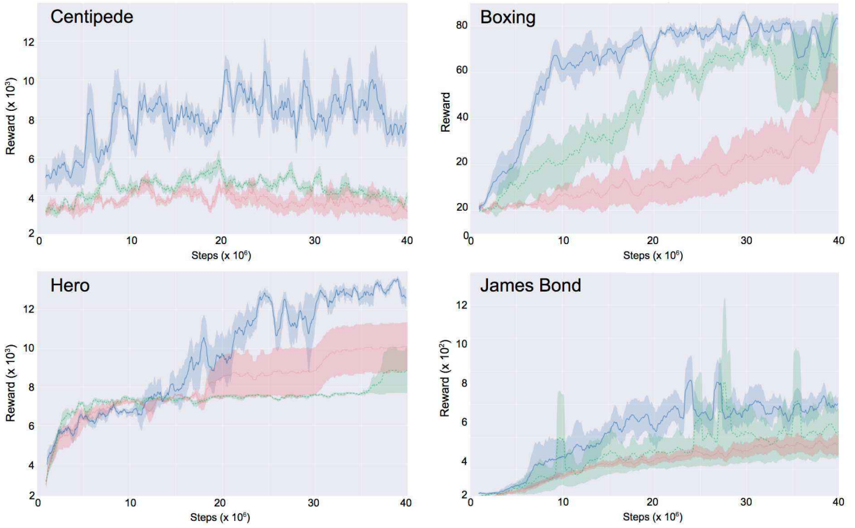
Figure 6: PathNet shows positive transfer from River Raid to Centipede, Boxing, Hero and James Bond. The graphs show the reward over the first 40 million steps of training. Blue shows the results from the best five hyperparameter settings of PathNet out of 243. Compare these to the best five hyperparameter setting runs for independent learning (red) and fine-tuning (green) controls out of 45.
