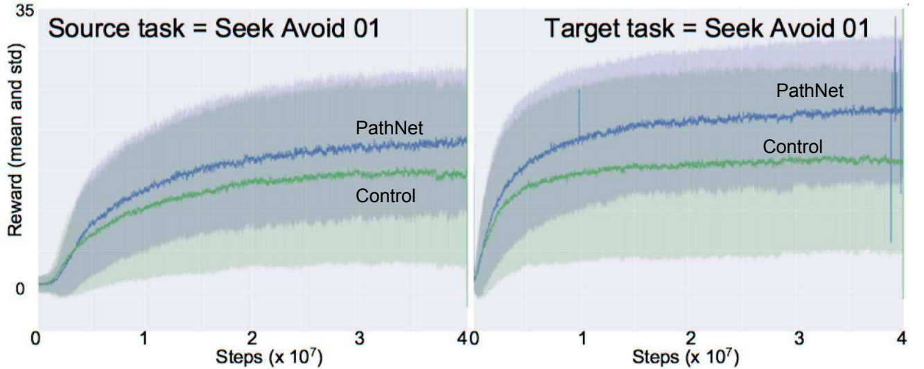
Figure 8: PathNet outperforms the de novo control and the fine-tuning control on learning seekavoid_arena for the first time, on average over all hyperparameters explored, out of 243 experiments. It also outperforms fine tuning when seekavoid_arena [10] is learned a second time, with a new value and policy readout, with the same set of 243 hyperparameter settings.
