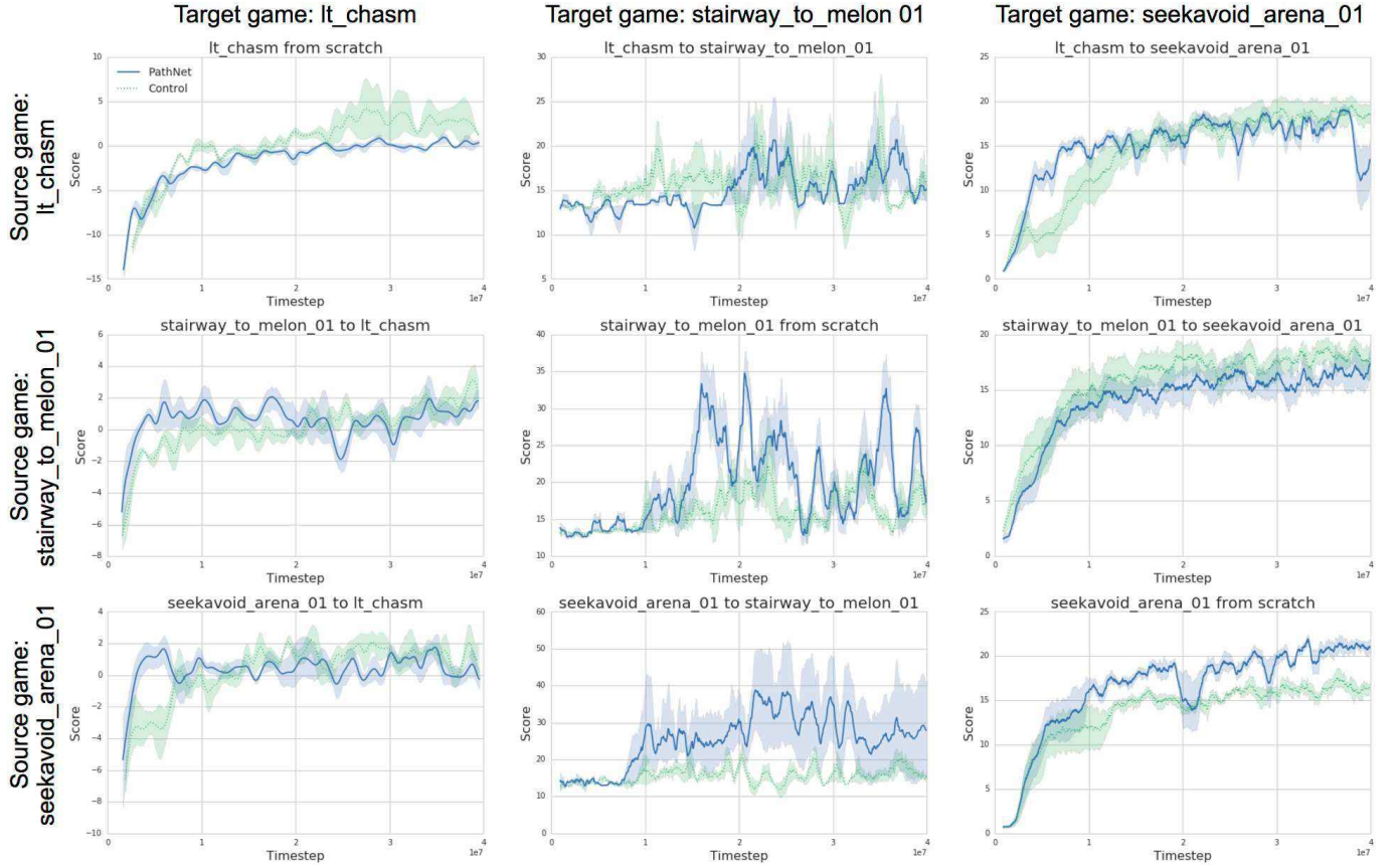
Figure 9: Means of the best 5 (out of a size 24 parameter sweep) training runs for PathNet compared with the fine-tuning (off diagonal) and independent path (diagonal) controls for the three Labyrinth levels considered. The diagonal results show the performance of PathNet when learning from scratch compared to the independent fixed path control. Off-diagonal results show the performance of pathNet during transfer.
