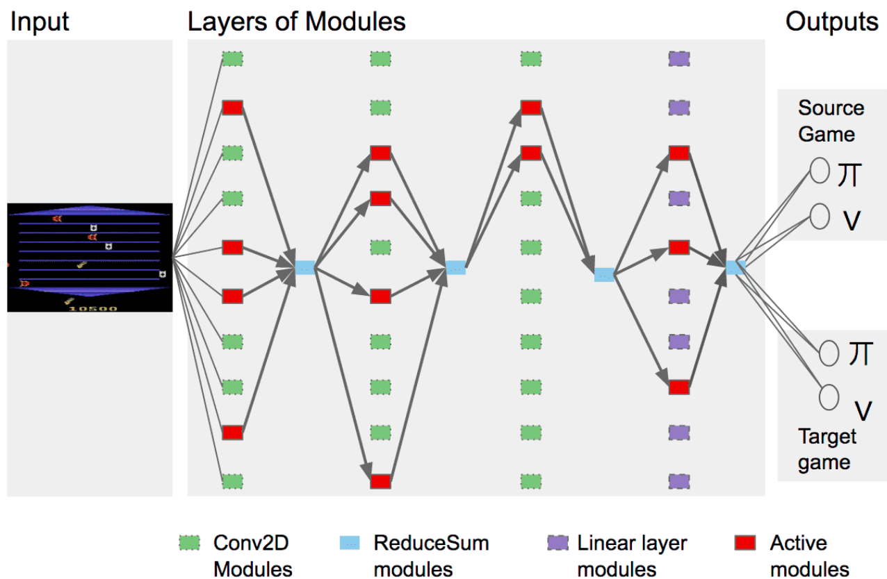
Figure 2: The PathNet used for learning Atari and Labyrinth games consists of a 4 layer network with 10 (or sometimes 15) modules in each layer. The first three layers' modules are convolutional 2D kernels with 8 kernels per module (green boxes in figure), kernel sizes (8, 4, 3), and strides (4, 2, 1) from 1st to 3rd layers respectively, and with the final layer consisting of fully connected linear layers of 50 neurons each (purple boxes). After each module there is a rectified linear unit. Between layers the feature maps are summed before being passed to the modules of the subsequent layer (blue boxes). Typically a maximum of 4 modules per layer are permitted to be included in a pathway (shown as red boxes), otherwise evolution would simply grow the pathway to include the whole network as this would improve fitness by growing the number of parameters that can be tuned by learning.
