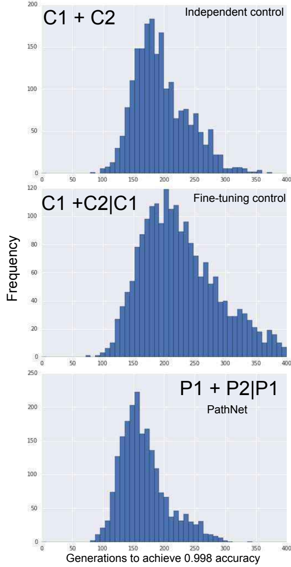
Figure 3: PathNet is capable of supporting transfer learning in binary MNIST classification. The top figure shows C1 + C2 which is the sum of learning times over the source and target tasks required to learn both tasks to 0.998 accuracy, with a separate maximum sized fixed path for each task, and thus constitutes the independent learning control; mean = 195 generations. The middle figure shows C1 + C2|C1 , which is the time required to learn both tasks where the second task is not learned from scratch, but by fine tuning the same maximum sized fixed path as was used to learn the first task; mean = 229 generations. The bottom graph shows the sum of times required to learn the source and target tasks using PathNet; mean = 167 generations.
