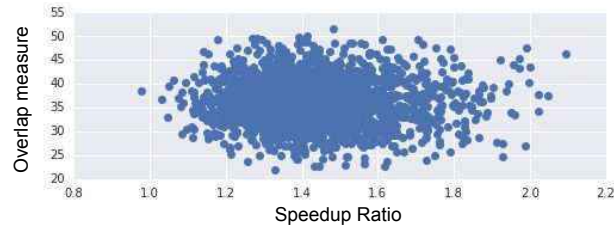
Figure 4: Overlap (y-axis) is not correlated with speedup ratio (C1 + C2)/(P1 + P2|P1) suggesting that PathNet discovers how much overlap to use based on whether the tasks could benefit from overlap or not.
