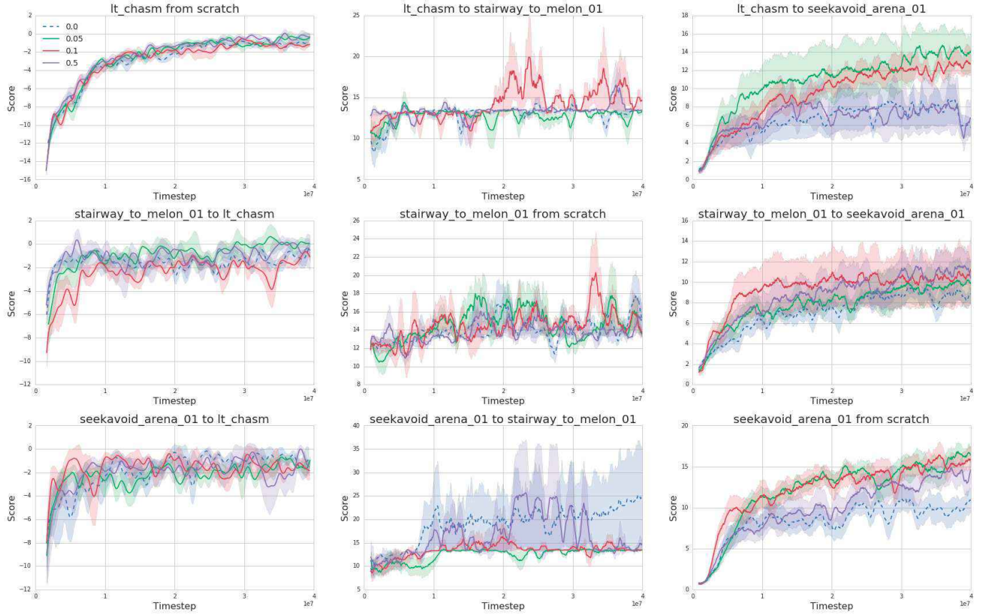
Figure 11: The contribution of Module Duplication on performance. Graphs show the mean performance across all hyperparameters for PathNet with different module duplication rates [0, 0.05, 0.1, 0.5] per episode completed by worker 0. For some tasks (e.g. learning seekavoid_arena module duplication has been beneficial).
