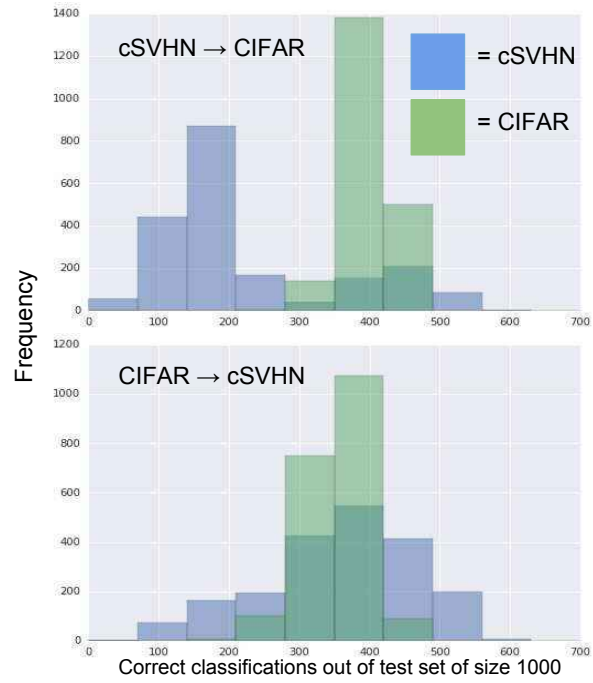
Figure 5: Top graph shows a histogram of accuracies when learning cSVHN first and CIFAR second. The bottom graph shows a histogram of accuracies when learning CIFAR first and cSVHN second. Learning either task second with PathNet results in improved performance, suggesting that PathNet is able to use weights in the optimal path found in task A, when learning task B.
