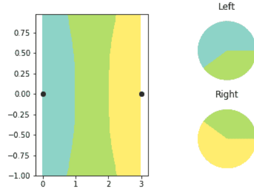
Figure 1: A SLaPkNN classifier is fitted on 2 soft-label prototypes and partitions the space into 3 classes. The soft label distribution of each prototype is illustrated by the pie charts.
