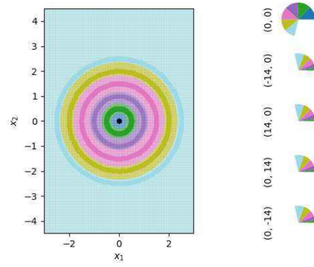
Figure 9: SLpKNN can separate 6 circles using 5 soft-label prototypes. Each pie chart represents the soft label of one prototype, and is labeled with its location. 4 of the prototypes are located outside of the visible range of the chart.
