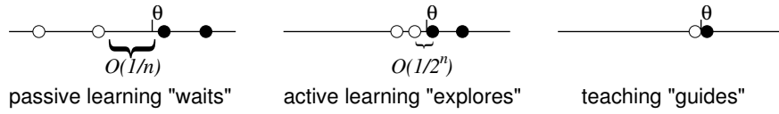
Figure 1: Teaching can require far fewer examples than passive or active learning
