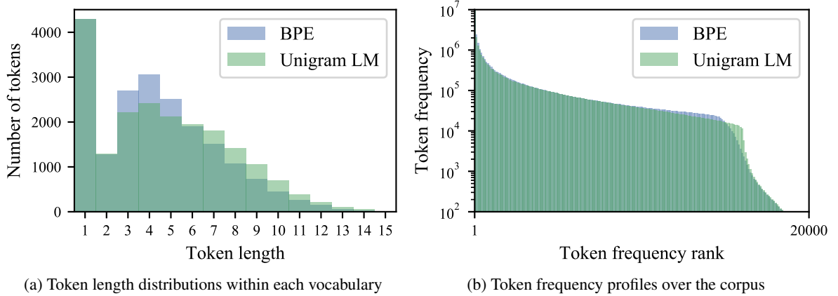
Figure 2: English subword vocabulary and corpus profiles. The unigram LM method produces longer tokens on average (a) and uses its vocabulary space more effectively (b), with more tokens of moderate frequency.
