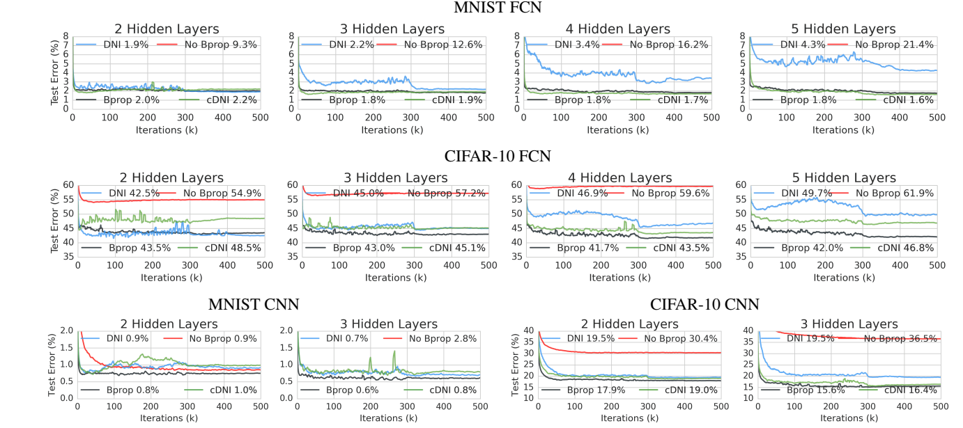
Figure 13. Corresponding test error curves during training for the results in Table 2. (a) MNIST digit classification with FCNs, (b) CIFAR-10 image classification with FCNs. DNI can be easily used with CNNs as shown in (c) for CNNs on MNIST and (d) for CNNs on CIFAR-10.
