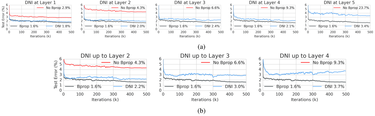
Figure 11. Test error during training of a 6 layer fully-connected network on MNIST digit classification. Bprop (grey) indicates traditional, synchronous training with backpropagation, while DNI (blue) shows the use of a (a) single DNI used after a particular layer indicated above, and (b) every layer using DNI up to a particular depth. Without backpropagating any gradients through the connection approximated by DNI results in poor performance (red).
