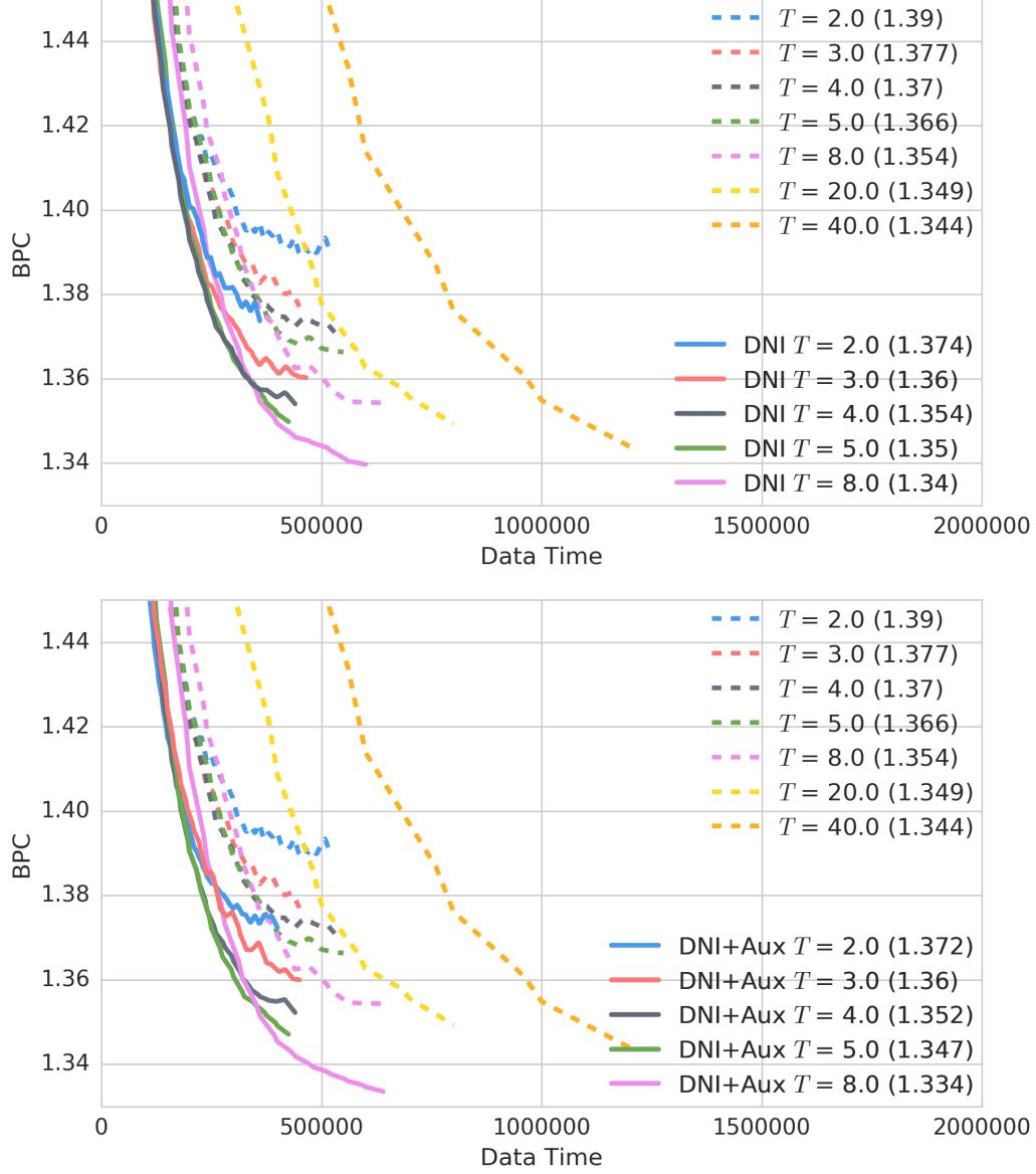
Figure 16. Test error in bits per character (BPC) for Penn Treebank character modelling. We train the RNNs with different BPTT unroll lengths with DNI (solid lines) and without DNI (dashed lines). Early stopping is performed based on the validation set. Top shows results with DNI, and bottom shows results with DNI and future synthetic gradient prediction (DNI+Aux). Bracketed numbers give final test set BPC.
