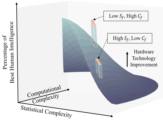
(c) Shocking the CIS: Role of CPU/GPU/TPU
