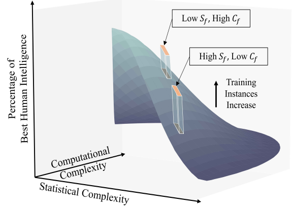
(b) Shocking the CIS: Role of Data
