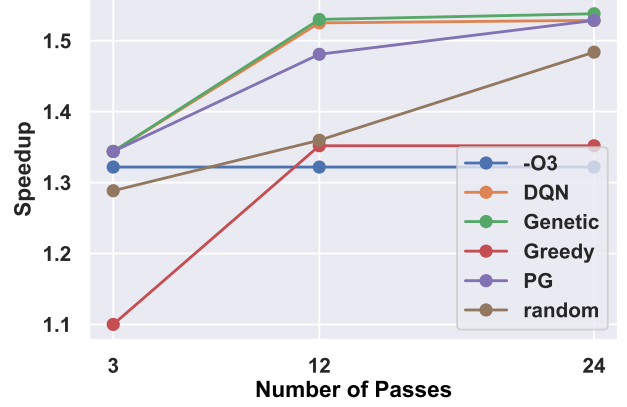
Fig. 1. Circuit speedup of various algorithms compared to No-Opt with sequence length of 3, 12, and 24.
