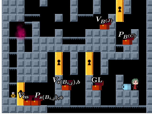
Figure 10: The B_{ij}^{(J)} rooms while they are in the jar chain. Note, relative to the room's initial state: (1) the ONE-TIME-TRAVERSAL gadget has been traversed, so the ring has been moved (e.g. by being thrown against the far right wall); (2) Rico has used the green flame, so it is gone (but Rico appears where it used to be); (3) Rico has dropped the jar containing the next B_{ij}^{(J)} room in the chain next to the re-entry point, for retrieval.
