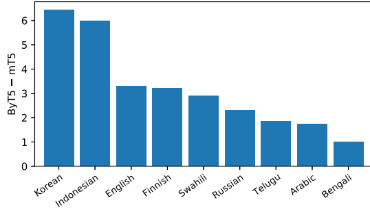
(a) TyDiQA-GoldP gap by language
