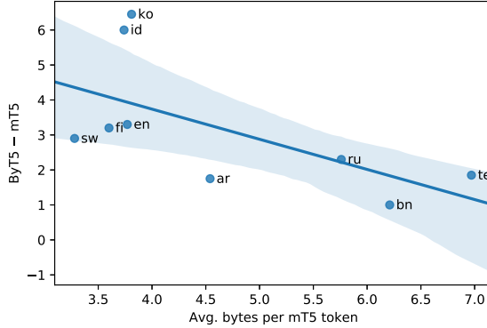
(c) TyDiQA-GoldP gap by compression
