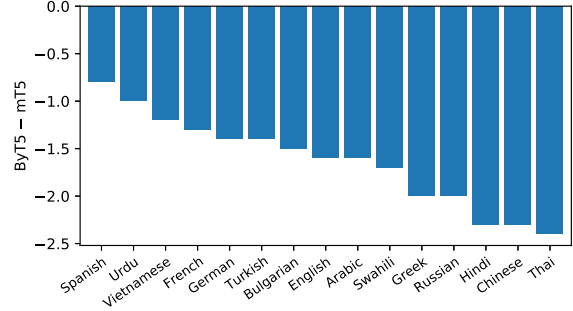
(b) XNLI gap by language
