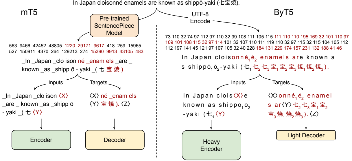
Figure 1: Comparison of pre-training example creation and network architecture between mT5 (Xue et al., 2020) and ByT5 (this work). mT5 : Text is split into SentencePiece tokens, spans of around 3 tokens are masked (red), and the encoder/decoder transformer stacks have equal depth. ByT5 : Text is processed as UTF-8 bytes, spans of around 20 bytes are masked, and the encoder is 3 times deeper than the decoder. Non-ASCII characters map onto multi-byte sequences. \langle X \rangle , \langle Y \rangle , and \langle Z \rangle represent sentinel tokens.
