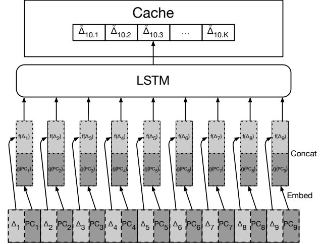
Figure 2. The embedding LSTM model. f and g represent embedding functions.
