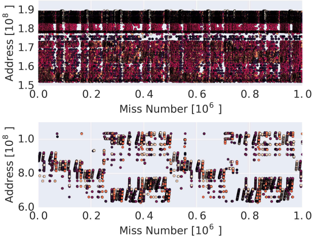
Figure 3. Two of six k-means clusters on the omnetpp benchmark dataset. Memory accesses are colored according to the PC that generated them.
