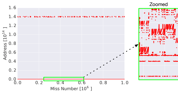
Figure 1. Cache miss addresses on the omnetpp dataset, demonstrating sparse access patterns at multiple scales.
