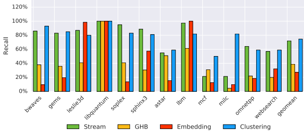
(b) Recall
