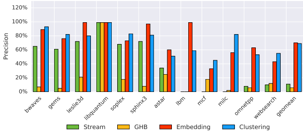
(a) Precision
