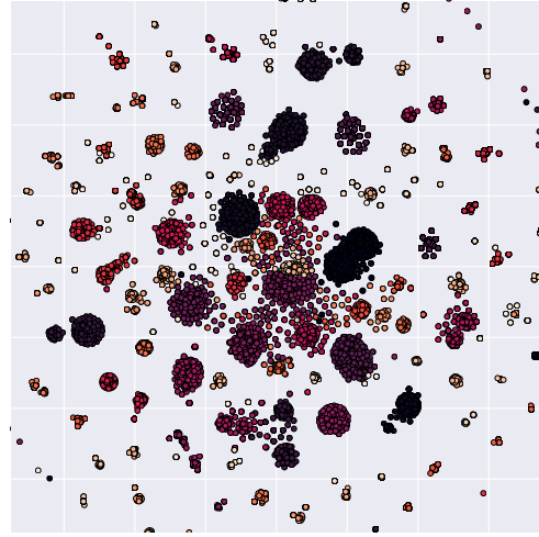
Figure 8. A t-SNE visualization of the concatenated ( \Delta , PC) embeddings on omnetpp colored according to PC instruction.
