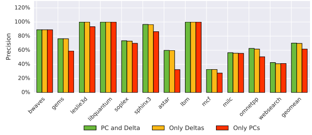
(a) Precision
