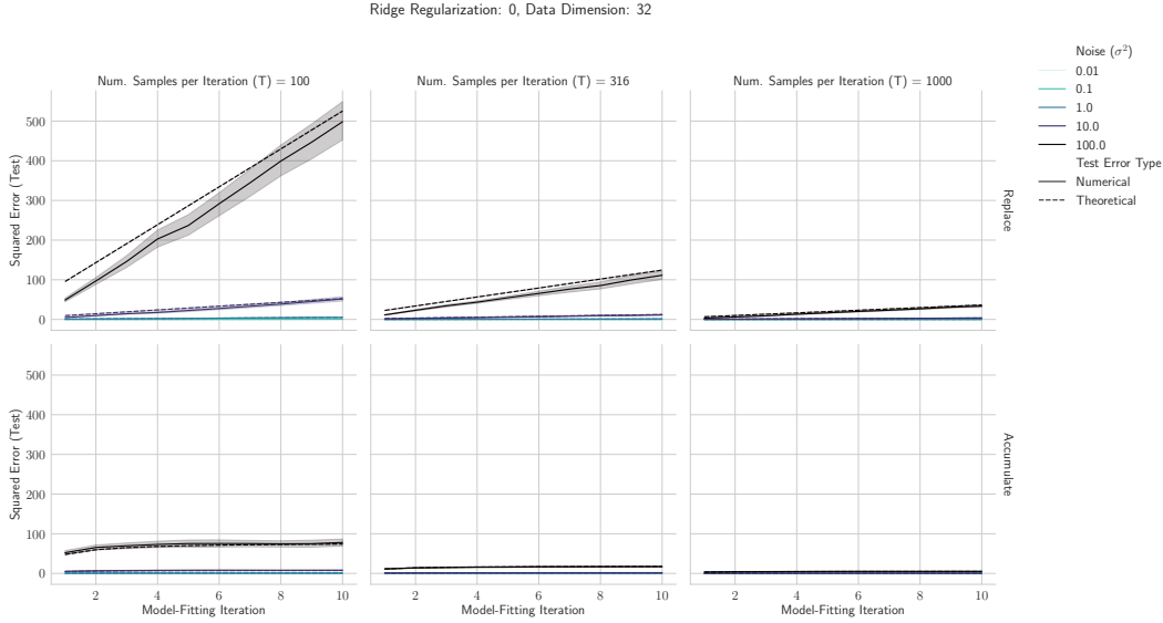
Figure 2: Accumulating Data Prevents Model Collapse in Linear Regression. We consider sequences of linear models recurrently fit to generated targets by previous iterations of models. Top: If each linear model is fit to the generated targets of only the preceding linear model, i.e., data are replaced, then the test error grows linearly with the number of iterations n . Bottom: If each linear model is instead fit to the generate targets of all the preceding linear models, i.e., data accumulate, then the test error has a finite upper bound independent of the number of iterations. This suggests that data accumulation might be a robust solution for mitigating model collapse. For log test error and higher iterations, see App. Fig. 9.
