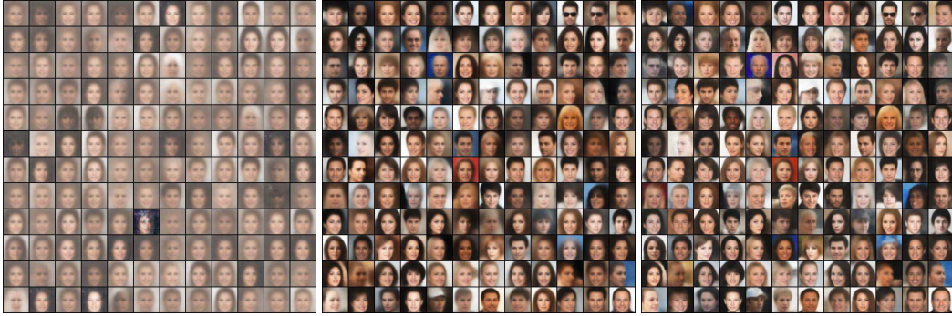
Figure 12: Data Accumulation Maintains Model Capabilities. Image reconstructions from the test set. Left: Training on prior iterations collapses the model’s capability, and subsequently, it can only represent a single mode. Middle: training on aggregated data preserves model capabilities and leads to little to no degradation in the reconstructed images. Right: Baseline reconstructions after 100 training epochs on the dataset.
