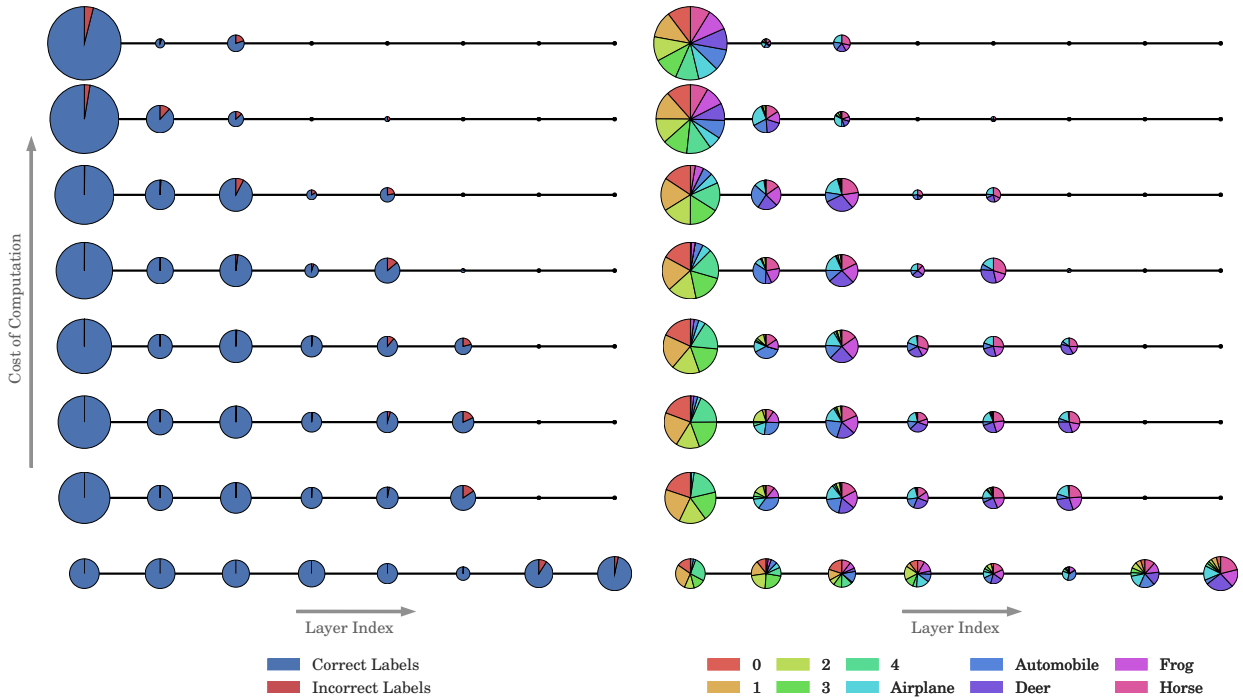
Figure 6. Dataflow through actor networks trained to classify images from the hybrid MNIST/CIFAR-10 dataset. Every row is a node-link diagram corresponding to a network, trained with a different k_{cpt} . Each circle indicates, by area, the fraction of examples that are classified at the corresponding layer. The circles are colored to indicate the accuracy of each layer (left) and the kinds of images classified at each layer (right).
