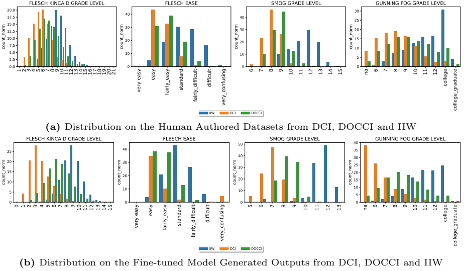
Fig. 13: Distribution-based Readability Metrics. We compare both human authored and model generated outputs from IIW and prior work to show the distribution of Education based units reflected in the writing style. IIW outputs from both the human annotators and the model produce a more mature style across the metrics.
