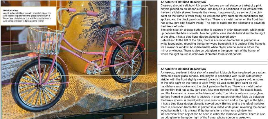
Fig. 11: IIW Final Annotation UI for Task-2. We illustrate the human annotations available from Task-1 as the human annotators hover over the salient objects in the image. The annotators can additionally switch between hiding all salient objects to view the image properly. Task-2 annotations starts with the seed caption from the VLM and is then refined by human annotators in sequential rounds, building on top of the previous round's output.
