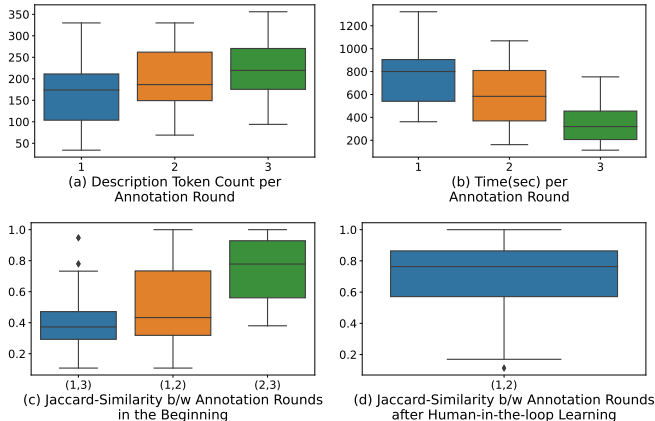
Fig. 2: Effects of Sequential Annotation: Over annotation rounds, (a) token count goes up as (b) time spent goes down with (c) higher agreement, measured by Jaccard Similarity [61]. A very low agreement across rounds (1,3) indicates considerable edits which annotators largely agreed upon in rounds (2,3). Round (1,2) provides the highest mean token count gain of \sim 30 . (d) Over time with a constant human annotator pool, each learns from the other via an implicit feedback loop and a high agreement rate in round (1,2) can now be observed as was previously only seen in round (2,3) in (c).
