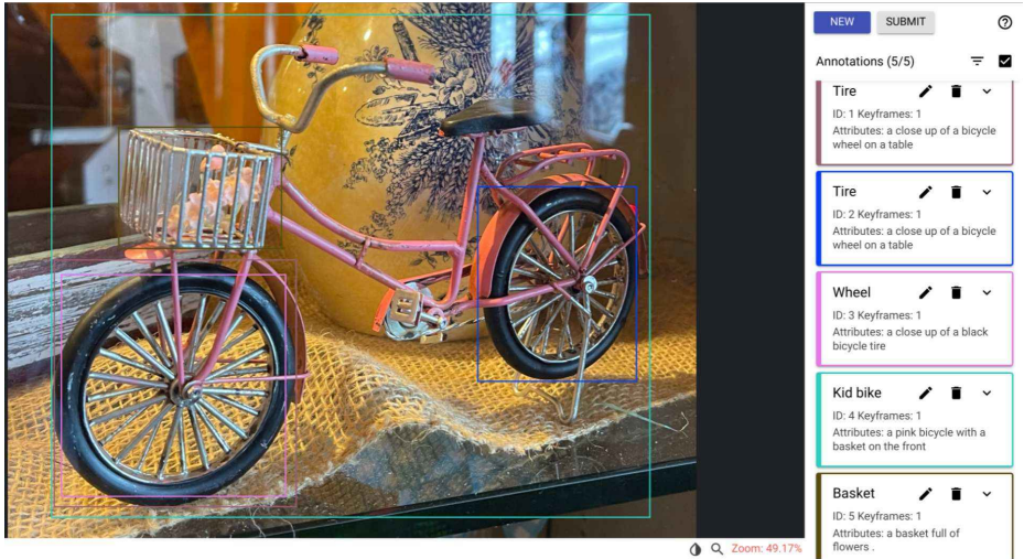
Fig. 8: IIW Annotation UI for Task-1. We illustrate the seed object-detection objects and VLM generated object-level captions with object cropped image bytes as input.
