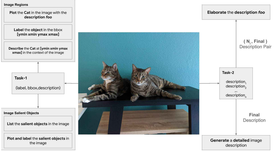
Fig. 12: IIW based VLM Fine-tuning Tasks. We show tasks based on data collected from Task-1 and Task-2 per the IIW annotation framework. Different tasks enable the fine-tuning to focus on the image at (object, attribute), (image, objects) or (image, hyper-detailed description) levels.
