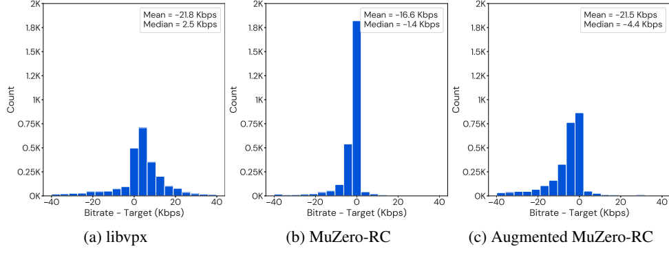
Figure 13: Histogram of overshoots of the agents on the evaluation set for 384 kbps target bitrate.
