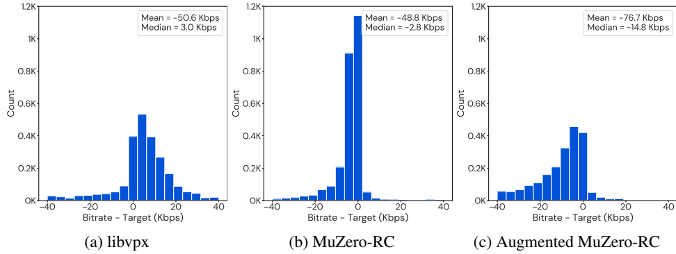
Figure 18: Histogram of overshoots of the agents on the evaluation set for 704 kbps target bitrate.
