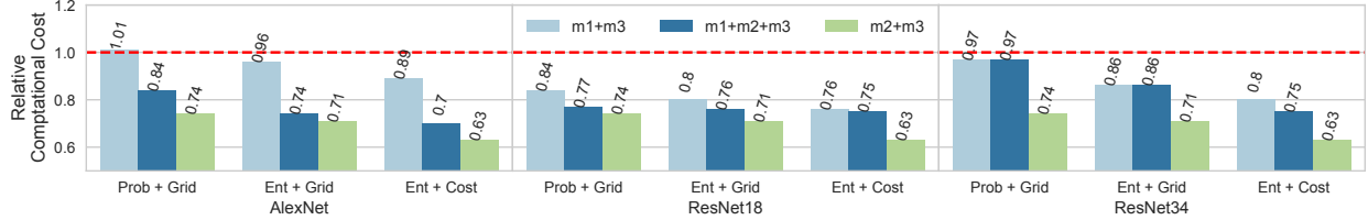
Figure 4: Three Model Cascade Results. We consider three element cascades m_1 \rightarrow m_2 \rightarrow m_3 where m_2 and m_3 are chosen to be the optimal two element cascade consisting of ResNet-50 and ResNet-152 respectively and we evaluate AlexNet, ResNet-18, and ResNet-34 as m_1 . We also evaluate each of the three IDK cascade designs and corresponding fitting procedure. In all cases, the accuracy is set to match that of ResNet-152 and we therefore only present the computational costs relative to the ResNet-152 model. In general we find that deeper cascades have diminishing returns due to increased evaluation costs
