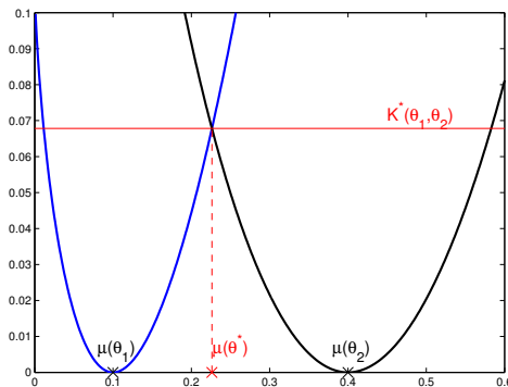
Figure 1: For Bernoulli distributions, the blue and black curves represent respectively \text{KL}(\mathcal{B}(\mu), \mathcal{B}(\mu_1)) and \text{KL}(\mathcal{B}(\mu), \mathcal{B}(\mu_2)) as a function of \mu . Their intersection gives the value of the Chernoff information between \mathcal{B}(\mu_1) and \mathcal{B}(\mu_2) , two distributions alternatively parameterized by their natural parameter \theta_1 and \theta_2 .
