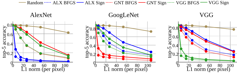
Figure 2: Accuracy when Varying the L_1 Norm per Pixel of the Perturbation. Accuracy for the three CNNs we evaluate. We denote the perturbation as XY , where X is the network that generated the perturbation — ALX (AlexNet), GNT (GoogLeNet), VGG — and Y indicates the BFGS perturbation or Sign . See Fig. 6 in A.1 for the same results using L_\infty .
