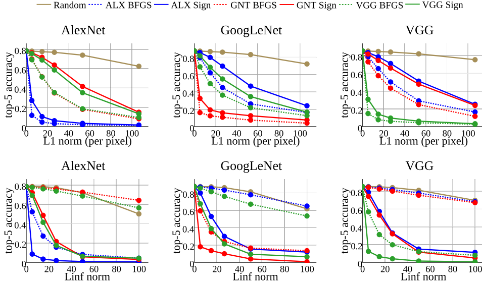
Figure 6: Accuracy when Varying the L_\infty Norm of the Perturbation. Accuracy for the three CNNs we evaluate. We denote the perturbation as XY , where X is the network that generated the perturbation — ALX (AlexNet), GNT (GoogLeNet), VGG — and Y indicates the BFGS or Sign .
