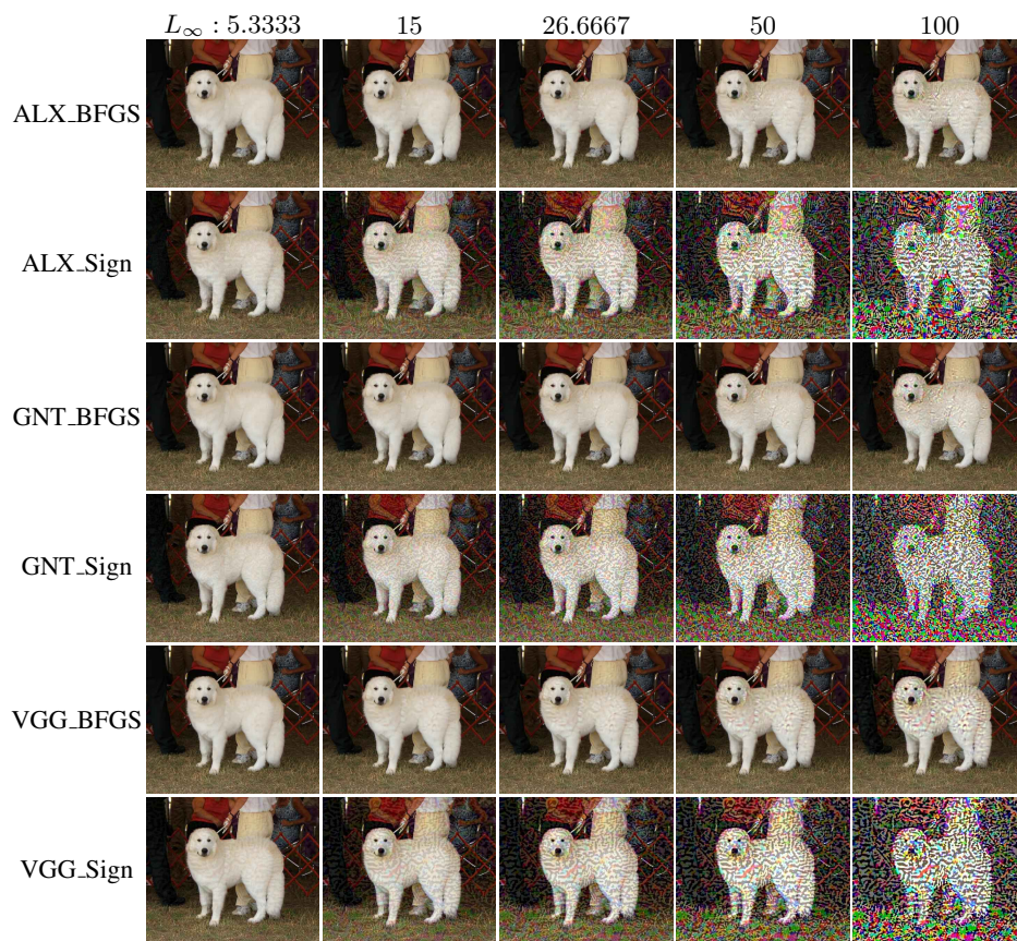
Figure 20: Qualitative example of the perturbations changing the average per pixel of the L_\infty norm. We denote the perturbation as X\ Y , where X is the network that generated the perturbation - ALX (AlexNet), GNT (GoogLeNet), VGG- and Y indicates the BFGS or Sign .
