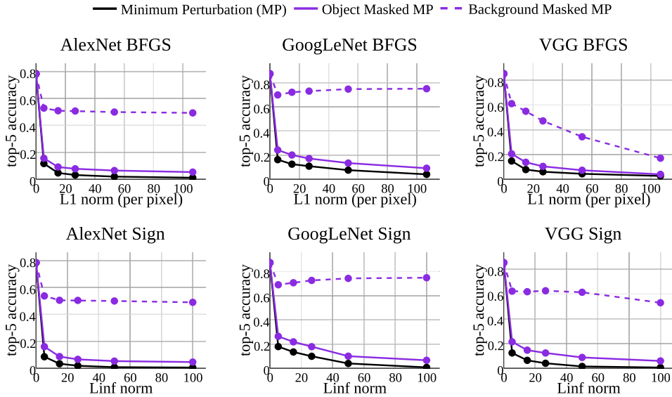
Figure 7: Accuracy of the Masked Perturbations. Accuracy for the three CNNs we evaluate, when varying the norm of BFGS (first row) and Sign (second row).
