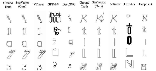
Figure 13. Baseline predictions on SVG-Fonts simplified test set
