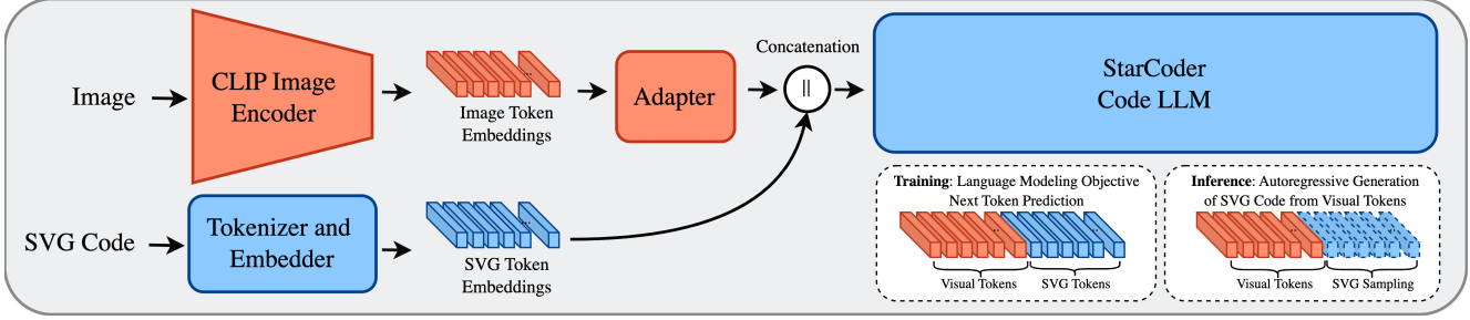
Figure 2. StarVector architecture: Images in the pixel space are encoded into a set of 2D embeddings using CLIP [56]. The Adapter applies a non-linear transformation to the image embeddings to align them with Code-LLM space, obtaining visual tokens. StarCoder uses the image embeddings as context to generate the SVG. During training the task is supervised by the next token prediction of the SVG tokens. During inference, the model uses the visual tokens from an input image to predict SVG code autoregressively.
