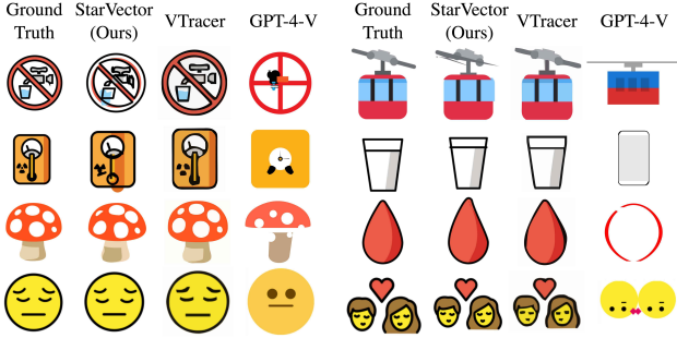
Figure 5. Results on SVG-Emoji test set
