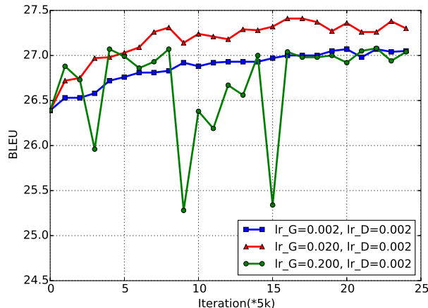
(a) D : Same learning rates; G : different learning rates.
