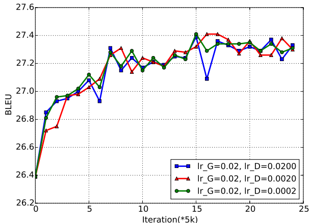
(b) G : Same learning rates; D : different learning rates.
