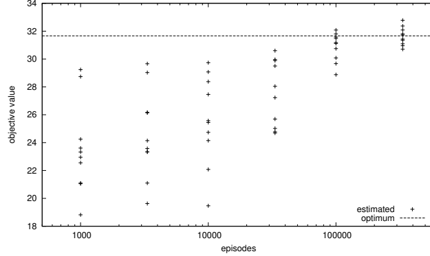
Fig. 2. Results for TD(0) on the SCP problem
