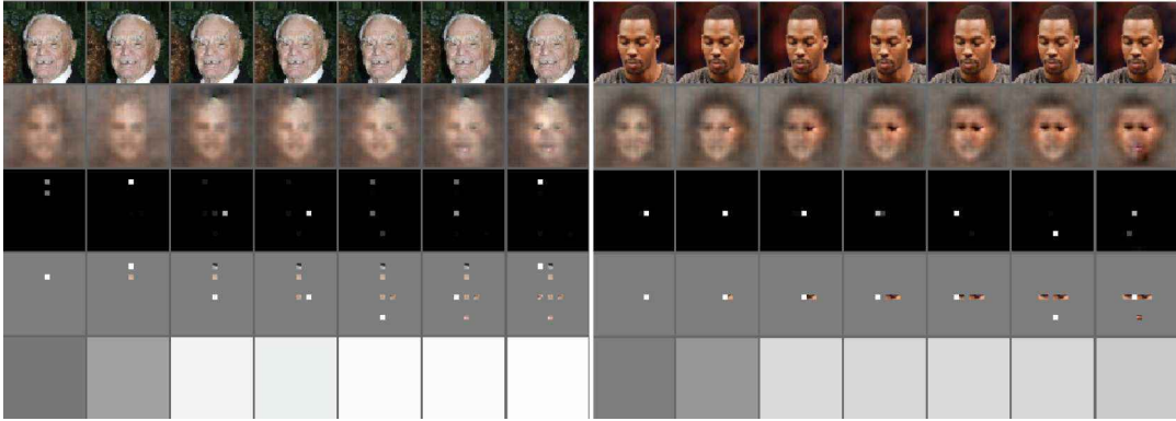
Figure 4: Conditional classification for CelebA (for a description of the rows, see Figure 3). In the left image, the model correctly guesses that the attribute “bald” is true. In right figure, the model makes a mistake about the attribute “narrow eyes”, even if it correctly identifies the most relevant part to discriminate the attribute.
