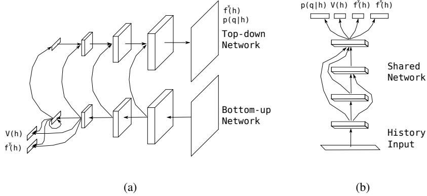
Figure 1: The network architectures developed for (a) our experiments with images and (b) our experiments with permutation-invariant data. We describe how computation proceeds through these architectures at each step of a trial in Section 3.4. The current trial history h_{:t} is input to (a) through the bottom-up network. The values f_{\theta}^x(h_{:t}) , f_{\theta}^y(h_{:t}) , V_{\theta}(h_{:t}) , and \pi_{\theta}(q_t|h_{:t}) are collected from the indicated locations. We use f_{\theta}^{x,y} to denote a model’s predictions about the complete observable data x and the unobservable data y . Computation in architecture (b) proceeds from bottom to top, starting with the history input h_{:t} and then passing through several fully-connected layers linked by shortcut connections. The values f_{\theta}^x(h_{:t}) , f_{\theta}^y(h_{:t}) , V_{\theta}(h_{:t}) , and \pi_{\theta}(q_t|h_{:t}) are computed as linear functions of the output of the shared network.
