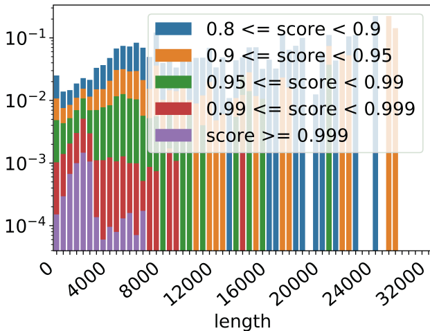
Figure 7: Fraction of documents with OpenAI detector score in different ranges as a function of untruncated character length. Low quality content tends to be shorter in length, peaking at 3000 characters.
