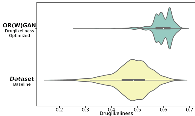
Figure 2: Violinplots of Druglikeness for molecules from the baseline Dataset (n=5000) and optimized OR(W)GAN (n=5440).
