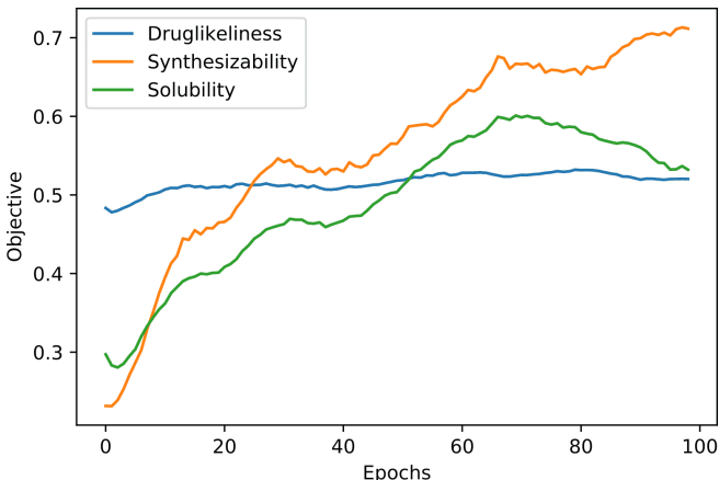
Figure 3: Plots of each objective across the training epochs. Objectives were trained for one epoch, and then switched for another.
