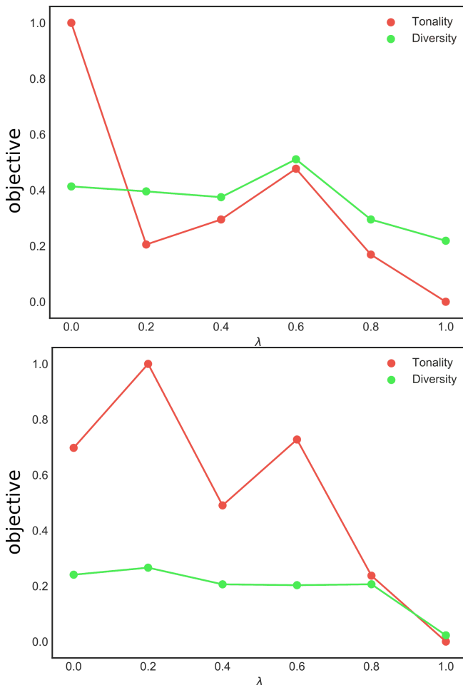
Figure 4: Plots of Diversity and Tonality rewards (the latter re-scaled to the [0, 1] interval) after 80 epochs of training on the music generation task. The upper plot employs the classical GAN loss, while the lower displays a WGAN. The values have been averaged over 1000 samples.
