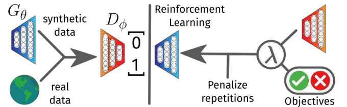
Figure 1: Schema for ORGAN. Left: D is trained as a classifier receiving as input a mix of real data and generated data by G . Right: G is trained by RL where the reward is a combination of D and the objectives, and is passed back to the policy function via Monte Carlo sampling. We penalize non-unique sequences.
