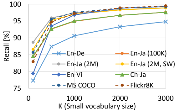
Figure 1: Recall scores of our vocabulary predictor.
