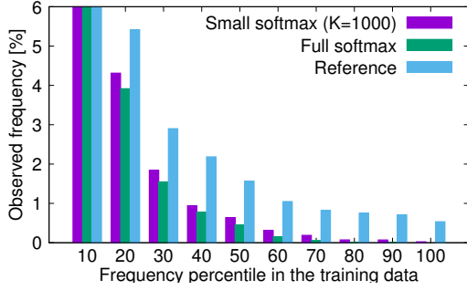
Figure 2: An analysis on the En-De translation results. The small and full softmax results are based on the REINFORCE setting, and “Reference” corresponds to the En-De reference translations of the development split.
