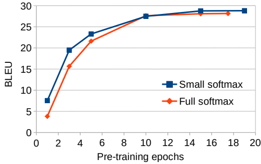
Figure 3: Effects of pre-training for REINFORCE.
