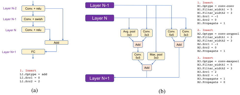
Figure 2: (a) An insert operation example for layer-by-layer search. (b) An insert operation example for module search. When the branch 3 is inserted, one of its source value is from branch 2. Once it is inserted, it cuts off the connection between branch 2 and the next layer, and sets “propagate” feature.
