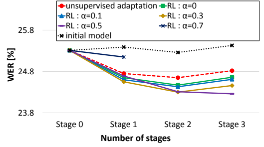
Fig. 2. Number of stages and WERs of the large batch data. At stage k , the RL k model is used to decode large batch \#k+1 .
