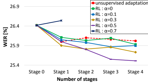
Fig. 3. Number of stages and WERs of the evaluation set.
