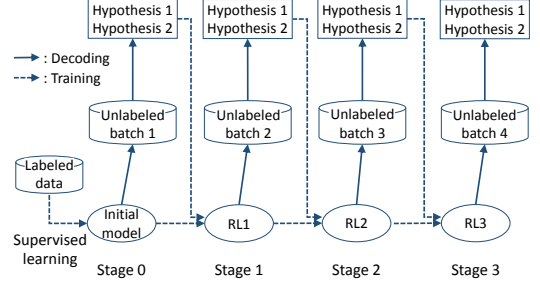
Fig. 1. Reinforcement learning process. RL k indicates a model made by applying reinforcement learning k times. RL k is made at stage k and used to decode large batch \#k+1
