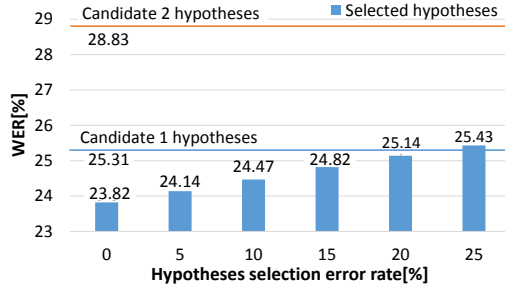
Fig. 4. Relationship between hypotheses selection error rate and WER of the selected hypotheses.
