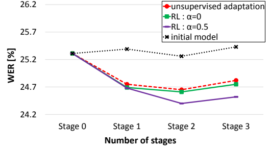
Fig. 5. Number of stages and WERs of the large batches when there is 15% hypotheses selection error.
