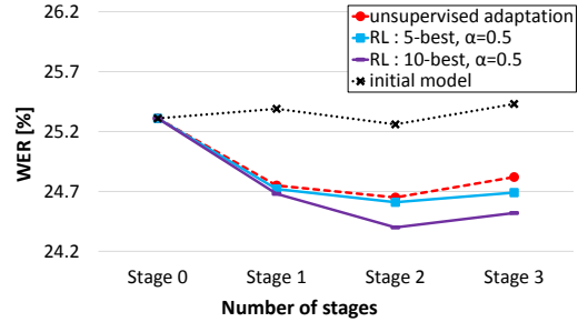
Fig. 6. Number of stages and WERs of the large batches when the 5th and 10th best hypotheses were used as the Candidate 2 results. 15% selection error rate is simulated.
