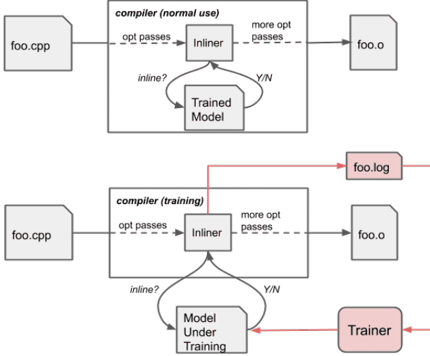
Figure 1. MLGO Overview
