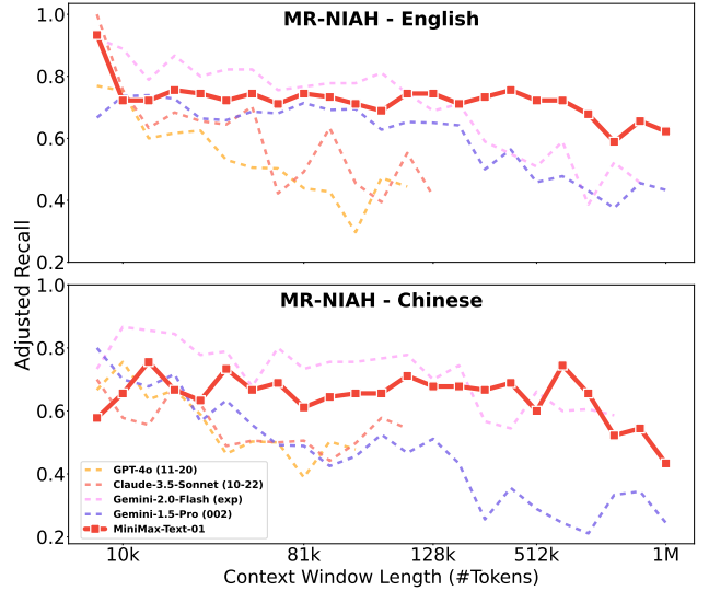
Figure 15 | MR-NIAH in English and Chinese.
