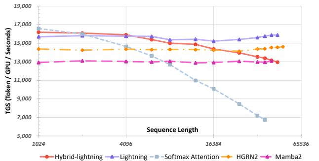
Figure 8 | The training speed of various attention mechanisms, including softmax, lightning, hybrid-lightning, HGRN2, and Mamba2, was benchmarked across sequence lengths ranging from 1,024 to 65,536. Performance was measured in terms of training speed, reported as tokens processed per GPU per second (TGS).
