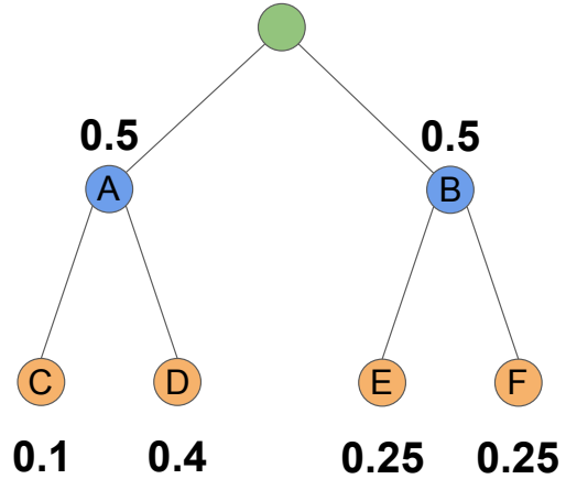
Figure 2. Any choice of temperature for local temperature sampling must have P(A) = P(B) . However, choosing global temperature \tau = 0.5 results in P(A) = 0.5763 and P(B) = 0.4237 which is impossible for any choice of local temperatures to satisfy.
