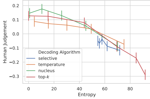
Figure 4. Human judgment scores as a function of decoding algorithm’s entropy. Each point represents a single choice of decoding algorithm and hyperparameter. Error bars represent 95% bootstrap confidence intervals.
