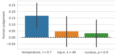
Figure 6. Human judgment scores for paired samples of equal log likelihood. 95% bootstrap confidence intervals. Dotted line represents random judgments. For all decoding strategies it can be seen that decreasing diversity tends to lead to higher-judged outputs.
