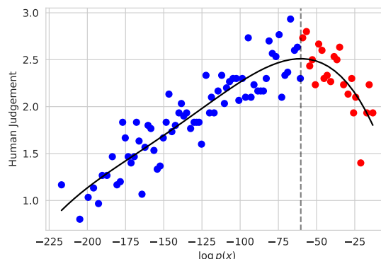
Figure 1. The Likelihood Trap. We asked 146 crowdworkers to rate the quality of 100 sentences across a variety of model likelihoods. While model log likelihoods are generally positively correlated with average human quality judgments, we notice an inflection point after which they become negatively correlated. Each point in the graph represents the average crowdworker rating of 5 sentences with similar model likelihoods. We discuss this phenomenon in more depth in Section 3.
