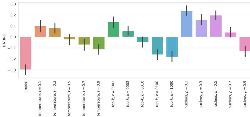
Figure 12. Human judgement scores for each decoding algorithm and hyperparameter choice, as measured in the inter-rater agreement experiment. Preference between sampling methods remains consistent with large-scale experiment shown in Figure 5 in spite of using only decodes generated by a subset of context sequences.
