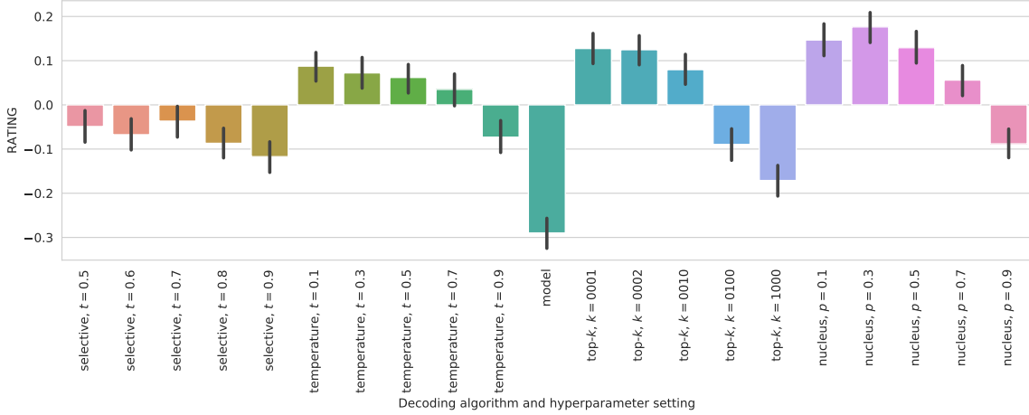
Figure 5. Human judgment scores for each decoding algorithm and hyperparameter choice. "Selective" is selective sampling and "model" is sampling directly from the probability distribution outputted by the language model. A score of 0 represents no preference. Selective sampling underperforms other more computationally efficient strategies.
