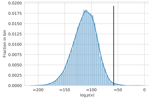
Figure 3. Histogram over p_{\text{model}}(x) for samples drawn from the same prompt. 99.5% of samples have log likelihood less than the chosen cutoff \alpha shown in black.
