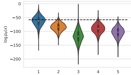
Figure 7. Distribution of prompt-conditional sample log likelihoods for five different prompts. The dotted-line represents the cutoff \alpha used in experiments.
