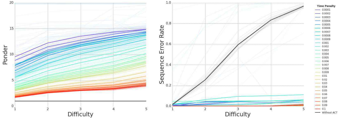
Figure 14: Addition Ponder Time and Error Rate Versus Input Difficulty. ‘Difficulty’ is the number of digits in each input vector; all sequences were length 3.
