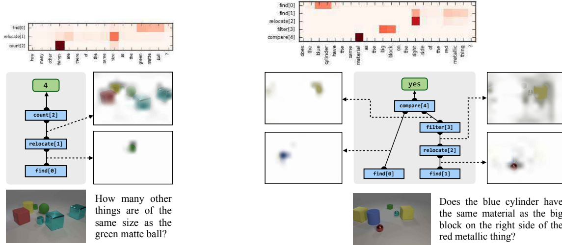
Figure 5: Question answering examples on the CLEVR dataset. On the left, it can be seen that the model successfully locates the matte green ball, attends to all the other objects of the same size, and then correctly identifies that there are 4 such objects (excluding the initial ball). On the right, it can be seen the various modules similarly assume intuitive semantics. Of particular interest is the second find module, which picks up the word right in addition to metallic red thing : this suggests that model can use the fact that downstream computation will look to the right of the detected object to focus its initial search in the left half of the image, a behavior supported by our attentive approach but not a conventional linguistic analysis of the question.
