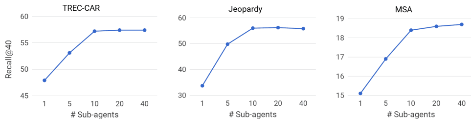
Figure 2: Overall system’s performance for different number of sub-agents.
