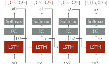
(b) Hyper-Parameter Policy Network
