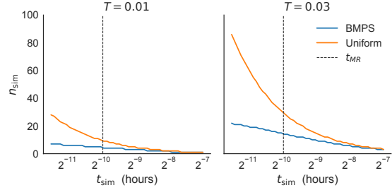
Figure 6: The number of simulations that can be run with versus without metareasoning as a function of the total time T and the cost of each simulation t_{\text{sim}} .
