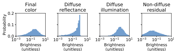
Figure 9. Distributions of brightness values in our disentangled image representation. We store our image data in an unnormalized HDR format, so we observe brightness values outside the range [0,1] . The horizontal axes in these plots are log-scaled.
