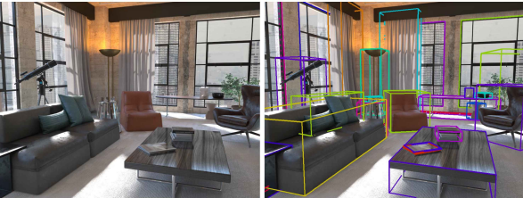
Figure 6. We include a tight 9-DOF bounding box for each semantic instance, so that our dataset can be applied directly to 3D object detection problems (e.g., [69]).
