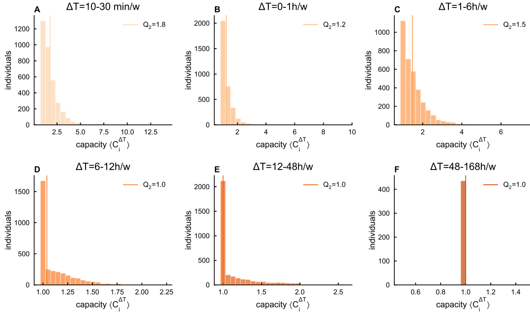
Supplementary Figure 29: CNS dataset: Composition of the AS. A-F) The distribution of the average individual capacity \langle C_i^{\Delta T} \rangle , considering locations seen for a time included in \Delta T .
