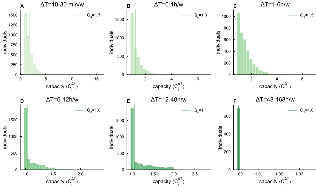
Supplementary Figure 30: MDC dataset: Composition of the AS. A-F) The distribution of the average individual capacity \langle C_i^{\Delta T} \rangle , considering locations seen for a time included in \Delta T .
