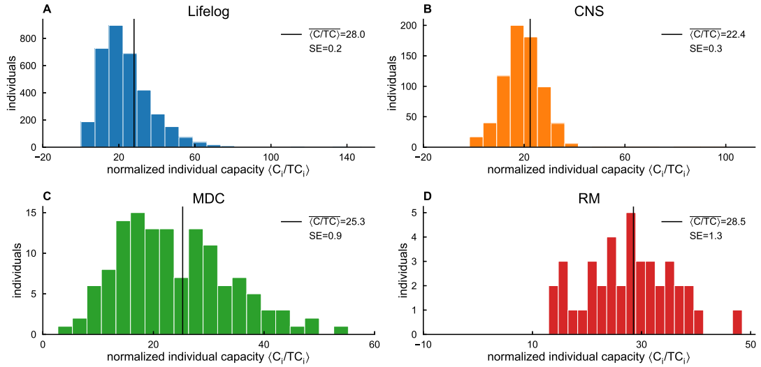
Supplementary Figure 18: Individual capacity: population homogeneity The frequency histogram of the normalized individual capacity \langle C_i/TC_i \rangle , where C_i and TC_i are respectively the location capacity and the time coverage of individual i . The average value \langle C/TC \rangle (black line) has standard error SE. Results are shown for the Lifelog (A), CNS (B), MDC (C) and RM (D), computed with W = 20 .
