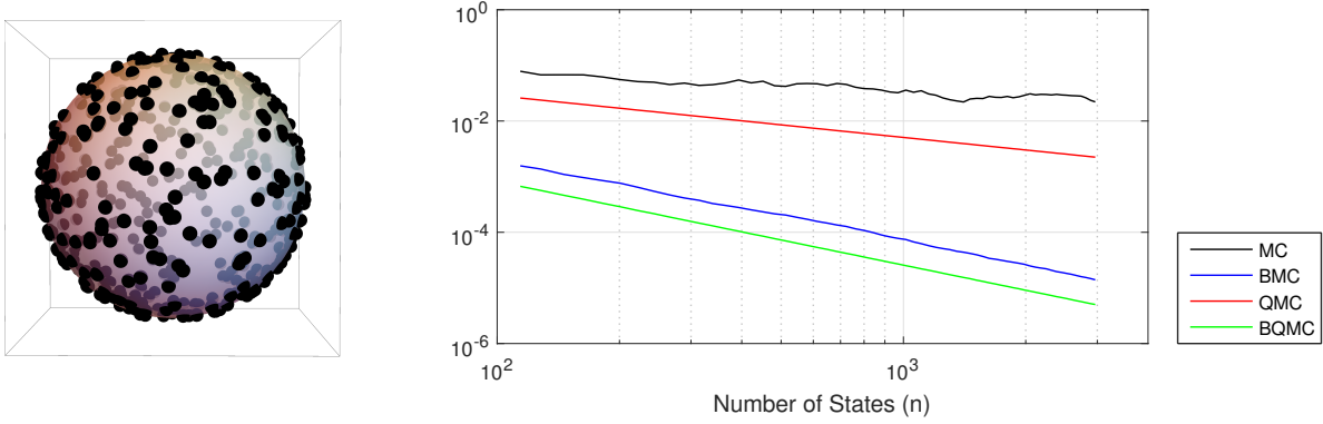
Figure 10: Application to global illumination integrals in computer graphics. Left: A spherical t -design over \mathbb{S}^2 . Right: The WCE, or worst-case-error, for Monte Carlo (MC), Bayesian MC (BMC), Quasi MC (QMC) and Bayesian QMC (BQMC).
