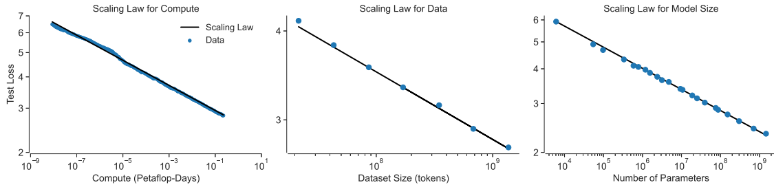
Figure 1 Scaling laws reliably predict that model performance (y-axes) improves with increasing compute ( Left ), training data ( Middle ), and model size ( Right ). In all cases a power-law (straight line, black) fits the empirically observed data (blue) exceptionally well. Figure adapted from [40].
