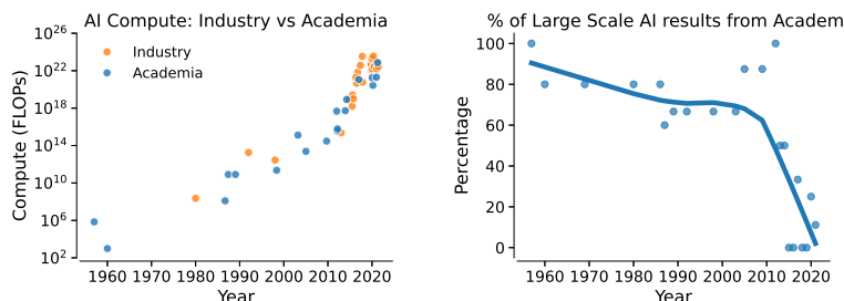
Figure 7 (Left) The amount of compute required by major AI projects over time is increasing exponentially for both academic (blue) and industrial (orange) projects. (Right) The proportion of computationally-intensive AI results from academia is steadily decreasing. (The blue curve represents a Lowess fit to the data.)
