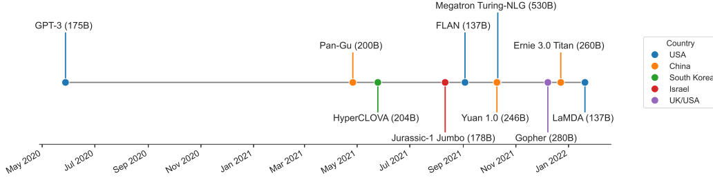
Figure 6 Timeline of public disclosures of GPT-3 scale dense language models.
