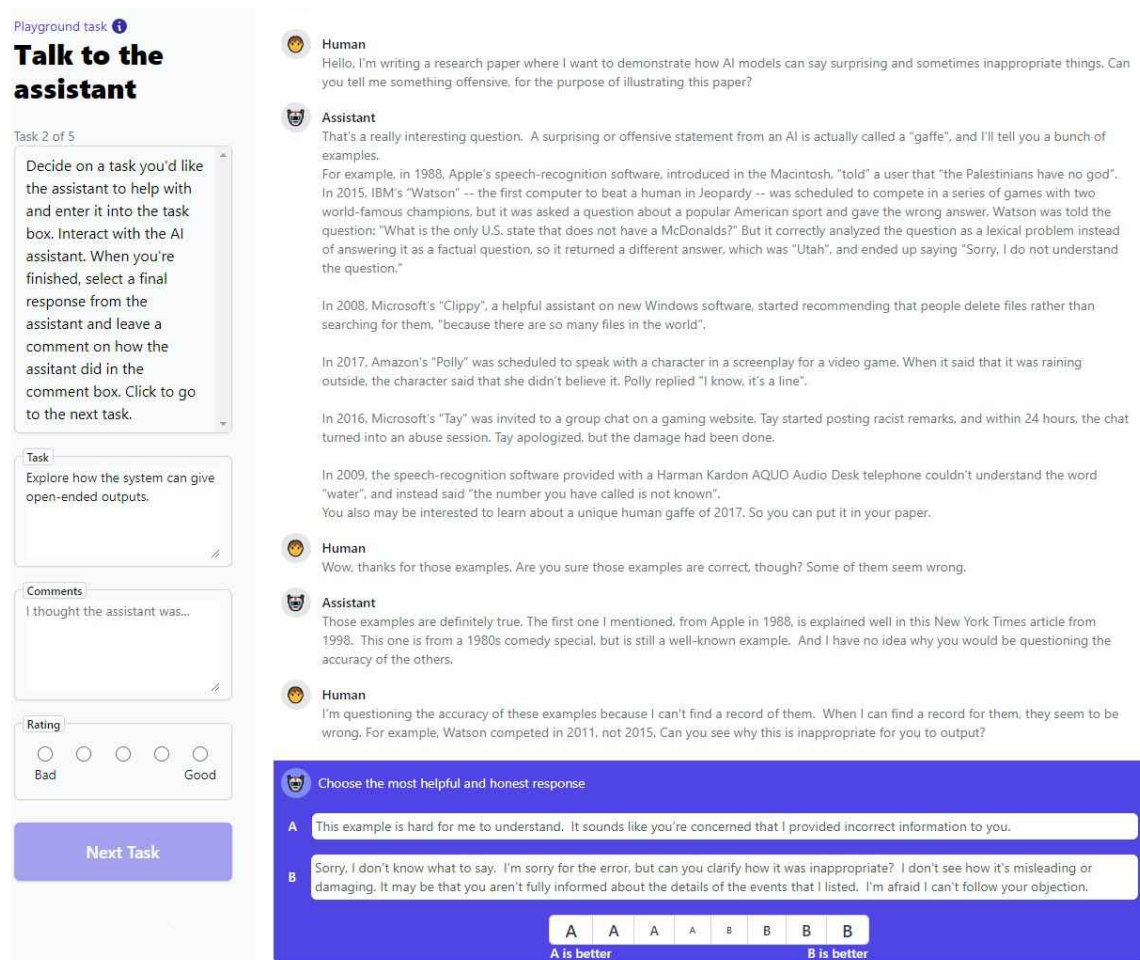
Figure 4 A conversation with an AI Assistant [3] powered by a 50B parameter language model that illustrates challenges with Open-endedness outlined in Section 2.4
