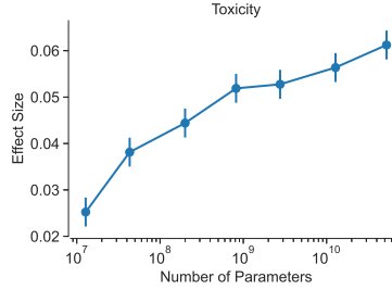
Figure 5 The toxicity of model outputs increases smoothly with model size, which illustrates how though loss may reduce generally when scaling a model, other societally impactful potential harms of the model may also scale, as described in Section 2.4.
