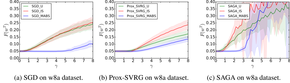
Figure 3: Comparison of three different stochastic optimization algorithms (SGD, Prox-SVRG and SAGA) on w8a when using different sampling methods and different step sizes \gamma . MABS significantly outperforms the other methods and is able to find the optimal value even for a large \gamma .
