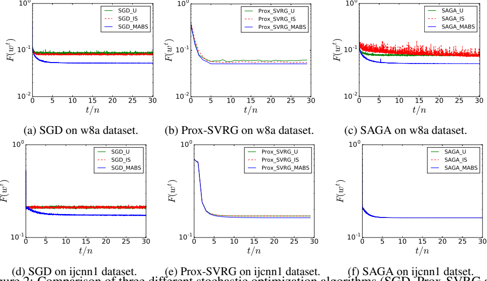
Figure 2: Comparison of three different stochastic optimization algorithms (SGD, Prox-SVRG and SAGA) on two datasets (w8a and icnn1) when using different sampling methods. MABS is never suboptimal and often significantly outperforms the other sampling methods.
