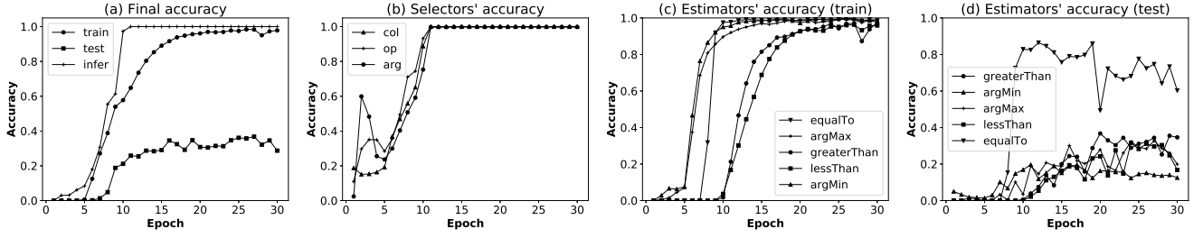
Figure 3: TAQ performance results - (a) Final accuracy in train, test, and inference modes. (b) Selector accuracy in train mode. (c) Estimator accuracy in train mode. (d) Estimator accuracy in test mode.
