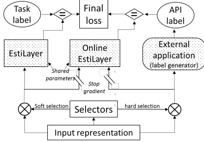
Figure 2: Label generation and online-training. We jointly optimize the model parameters with respect to the task label (left side) and the EstiLayer parameters with respect to the application label (middle and right side). We stop the gradients flow while optimizing the EstiLayer parameters with respect to the application label, and thus enforce it to retain application functionality. Note that 1) the EstiLayer and the online EstiLayer share their parameters and 2) the API label is generated online from the input to the EstiLayer and not from the task input.
