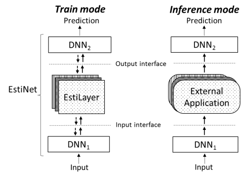
Figure 1: The Estimate and Replace approach: Train - Use an EstiLayer to estimate an external functionality and train an EstiNet DNN model end-to-end. Inference - Replace the each EstiLayer with an external application to achieve optimal results. A rectangle represents a neural network and a rectangle with rounded corners represent an external application. Solid arrows are for the forward pass and dashed arrows are for the back propagation flow.
