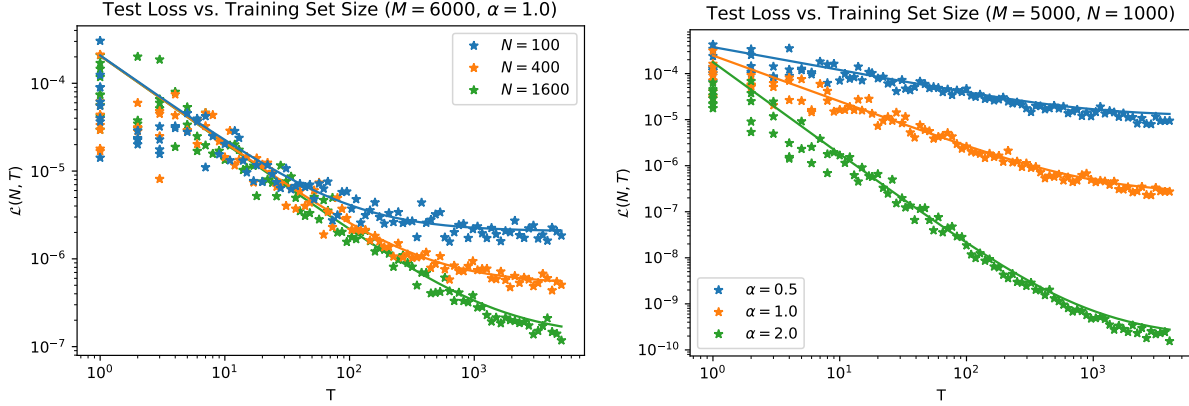
Figure 7: Test loss from numerical simulations (stars) of our optimally regularized ( \gamma = \gamma^* ) joint statistical model ( \sigma_u^2 = 1 , \lambda_+ = 1 , \sigma_w^2 = 1 , \sigma_\epsilon^2 = 0 ) as a function of training set size demonstrating the same rich behavior as LLMs and a simple fit (solid lines) given by (41): analogous to Fig. 1, if the model isn't bottlenecked by the number of parameters, N \rightarrow \infty , the test loss behaves as a power law in the training set size, \mathcal{L}(N, T) \sim T^{-\alpha} ; otherwise, if the number of parameters is too small for a given training set, then the test loss stalls at a plateau at a value that depends predictably on the parameters, \mathcal{L}(N, T) \sim N^{-\alpha} . Similar statements would hold if we plotted the test loss as a function of the number of features. (For smaller values of T , the variance of any particular realization is large, and so we've plotted multiple simulations for T \lesssim 10 .) Left: The size of the training set, T , is varied for a few different sized models, N , while the size of the latent space and the power-law exponent is held fixed ( M = 6000 , \alpha = 1.0 ). Right: The size of the training set, T , is varied for a few different power-law exponents, \alpha , while the size of the latent space and the size of the model is held fixed ( M = 6000 , N = 1000 ).
