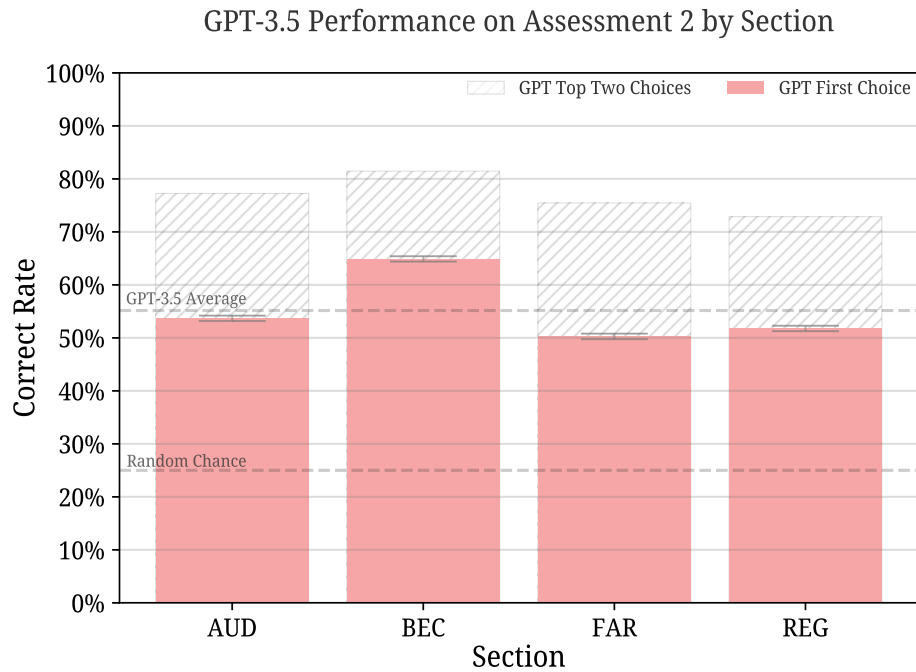
Figure 1: Performance of GPT-3.5 by section of AICPA Exam Blueprints for best prompt and parameter, with correct rate including second-best answer in dashed region. Error bars are \pm 1 standard error of the mean. Note that GPT-3.5 is not assessed on Analysis or Evaluation tasks, unlike human test-takers, and that the percentage of questions correct does not scale linearly with score or passage.
