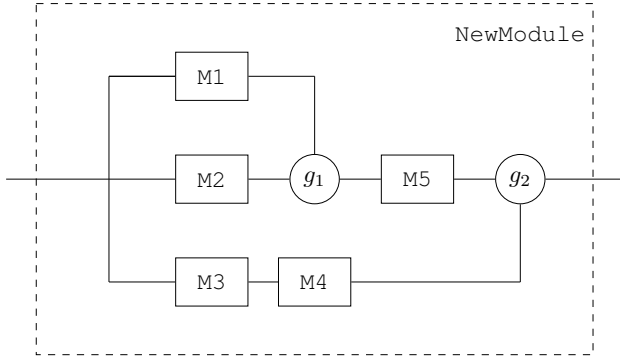
Figure 10. A module with many signal paths from input to output. To implement a module, the human expert only needs to implement its module interface. M1 , M2 , M3 , and M4 are arbitrary single-input single-output modules; g_1 and g_2 are arbitrary transformations that may have additional hyperparameters. The hyperparameters of g_1 and g_2 can be managed internally by NewModule .
