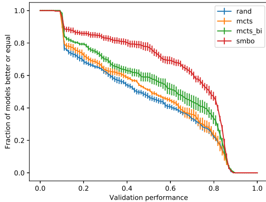
Figure 6. Percentage of models above a given validation threshold performance. MCTS with bisection and SMBO outperform random search. when compared to random search. The error bars have size equal to the standard error.
