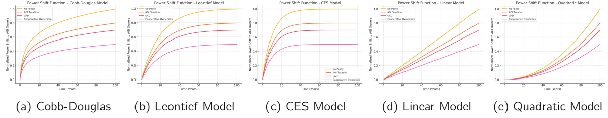
Figure 2: Impact of Policy Interventions on AGI Power Accumulation: This figure presents the effect of taxation, Universal AI Dividends (UAD), and cooperative ownership on normalized power shift functions across various economic models. Elastic models (Cobb-Douglas, CES) exhibit a more gradual power shift reduction under taxation, whereas rigid models (Leontief, Quadratic) show inherent constraints on AGI expansion. Cooperative ownership proves most effective in preventing rapid AGI dominance, while taxation slows but does not fully reverse power concentration.
