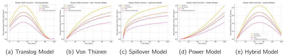
Figure 3: Continuation of Policy Impact Analysis on AGI Power Accumulation: This figure further illustrates how policy interventions shape AGI dominance in alternative economic models. The Spillover and Hybrid models show that cooperative ownership and taxation significantly influence long-run power dynamics, while the Power Model reveals that extreme wealth concentration persists despite interventions. The Von Thünen model exhibits diminishing returns that naturally limit AGI's expansion, reinforcing the role of structural economic constraints.
